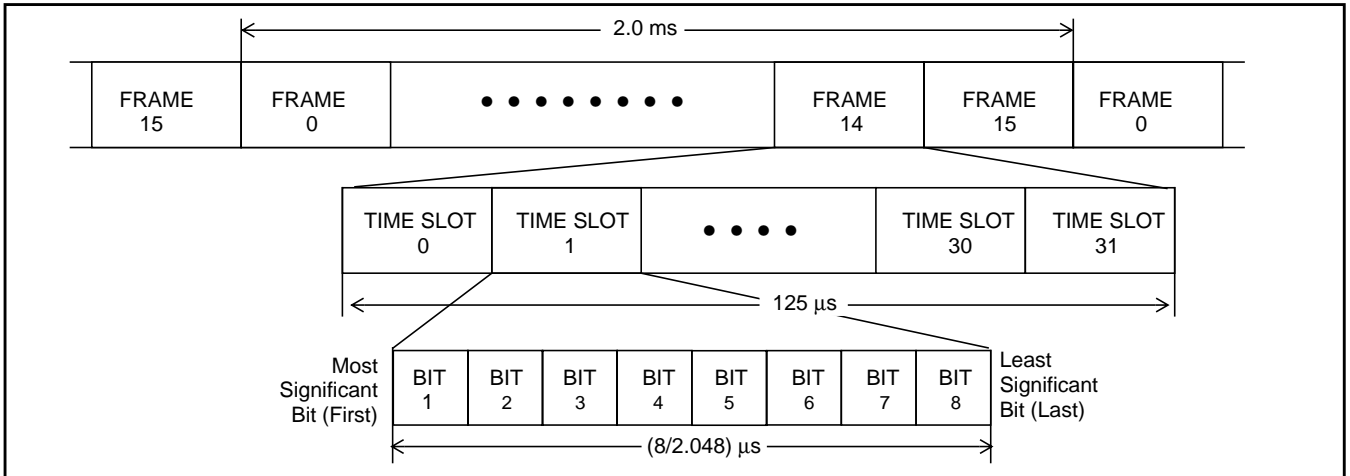
Figure 43 - PCM 30 Format
