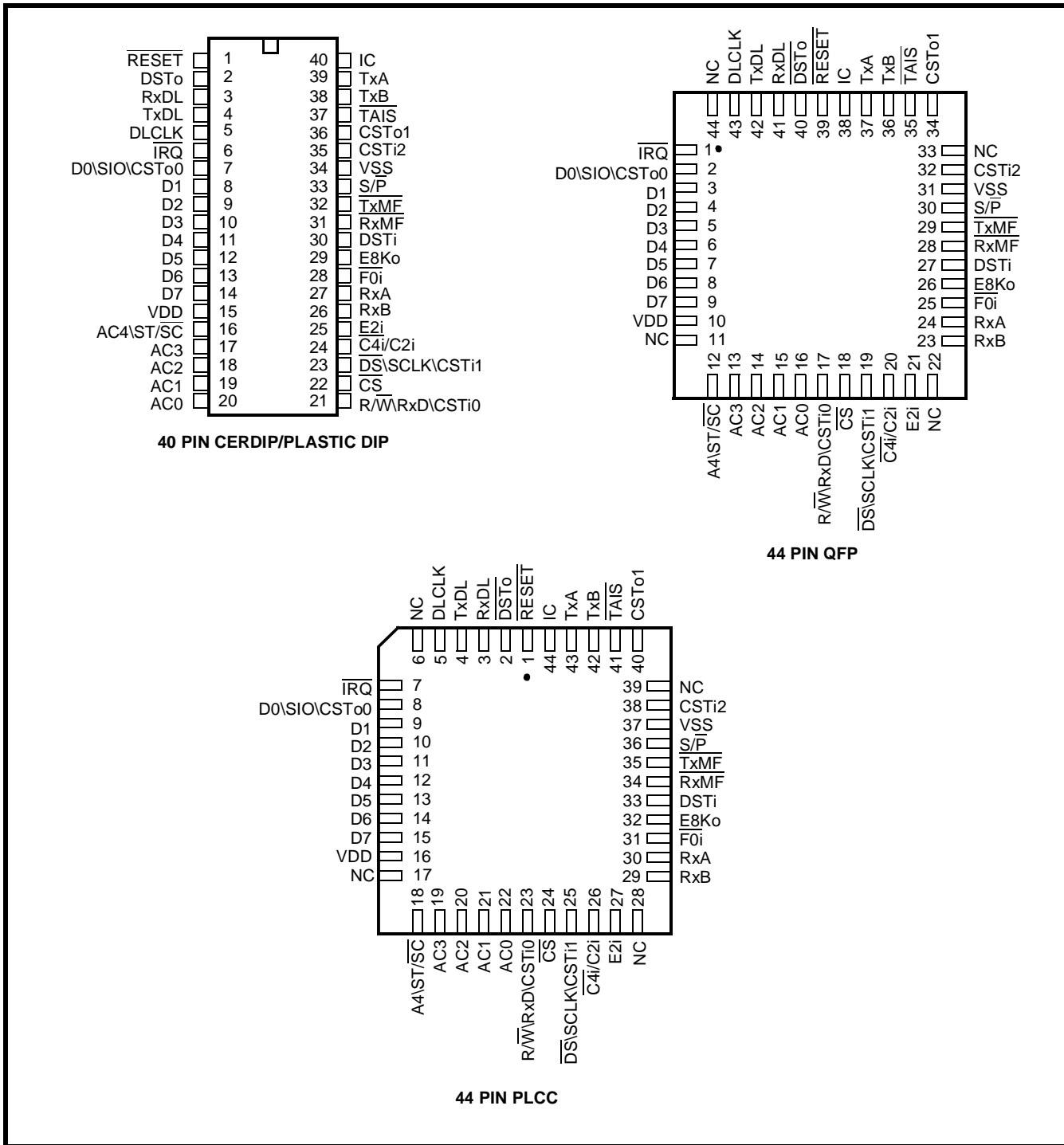
Figure 2 - Pin Connection
