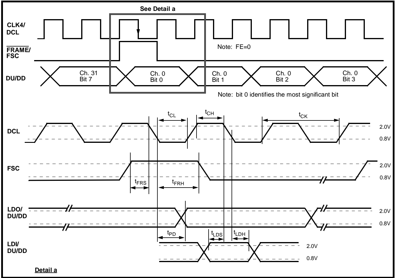
Figure 20 - GCI Timing
