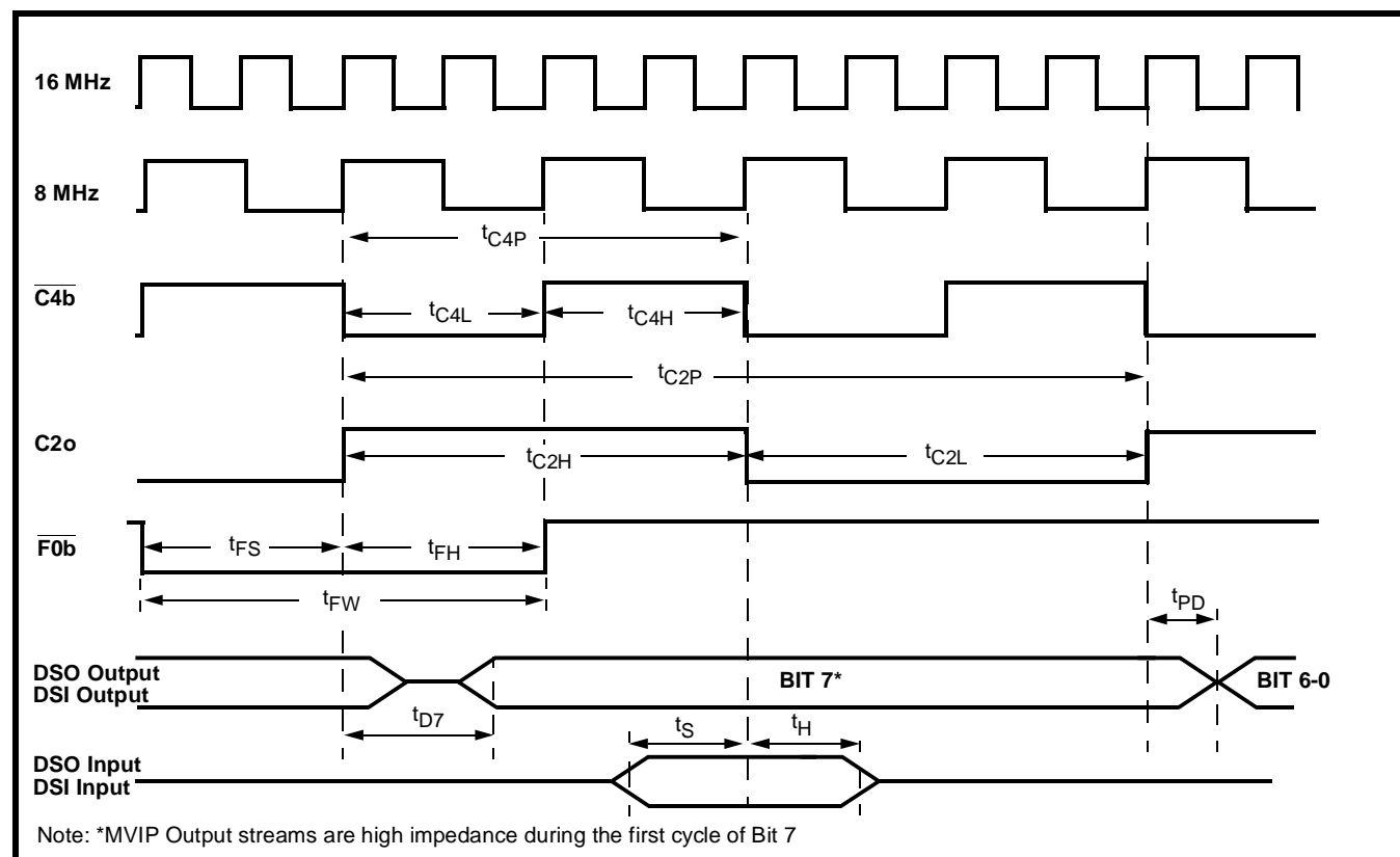
Figure 13 - MVIP Stream Timing
