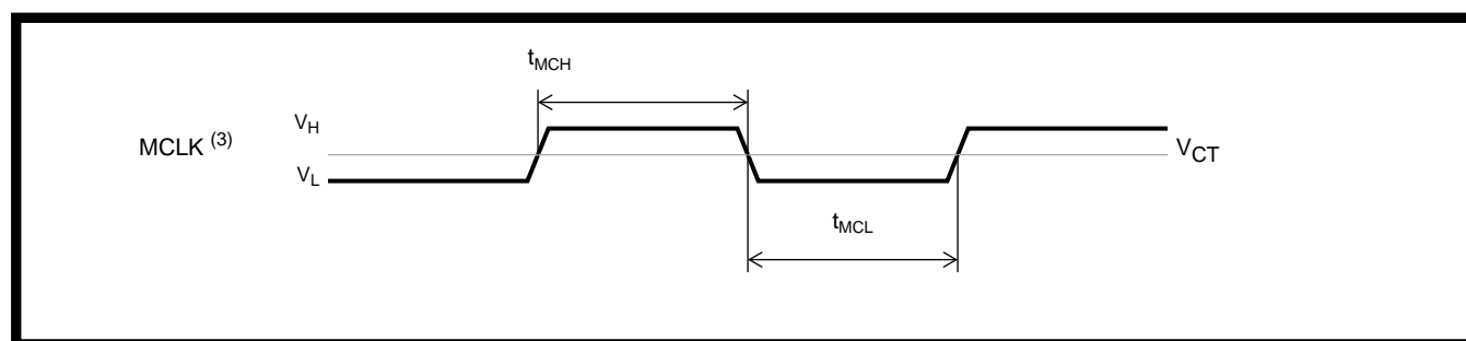
Figure 16 Master Clock - MCLK
