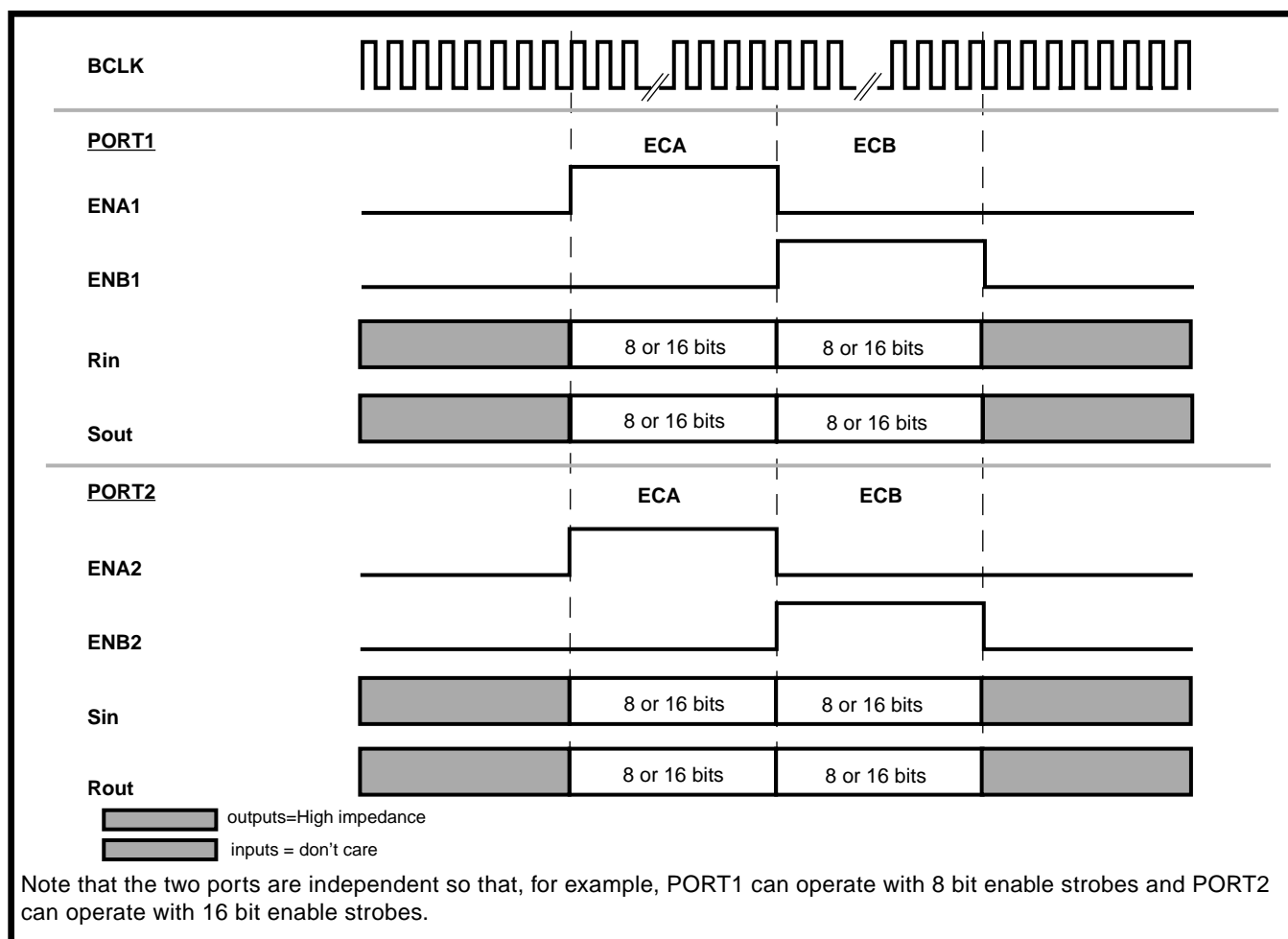
Figure 9 - SSI Operation
