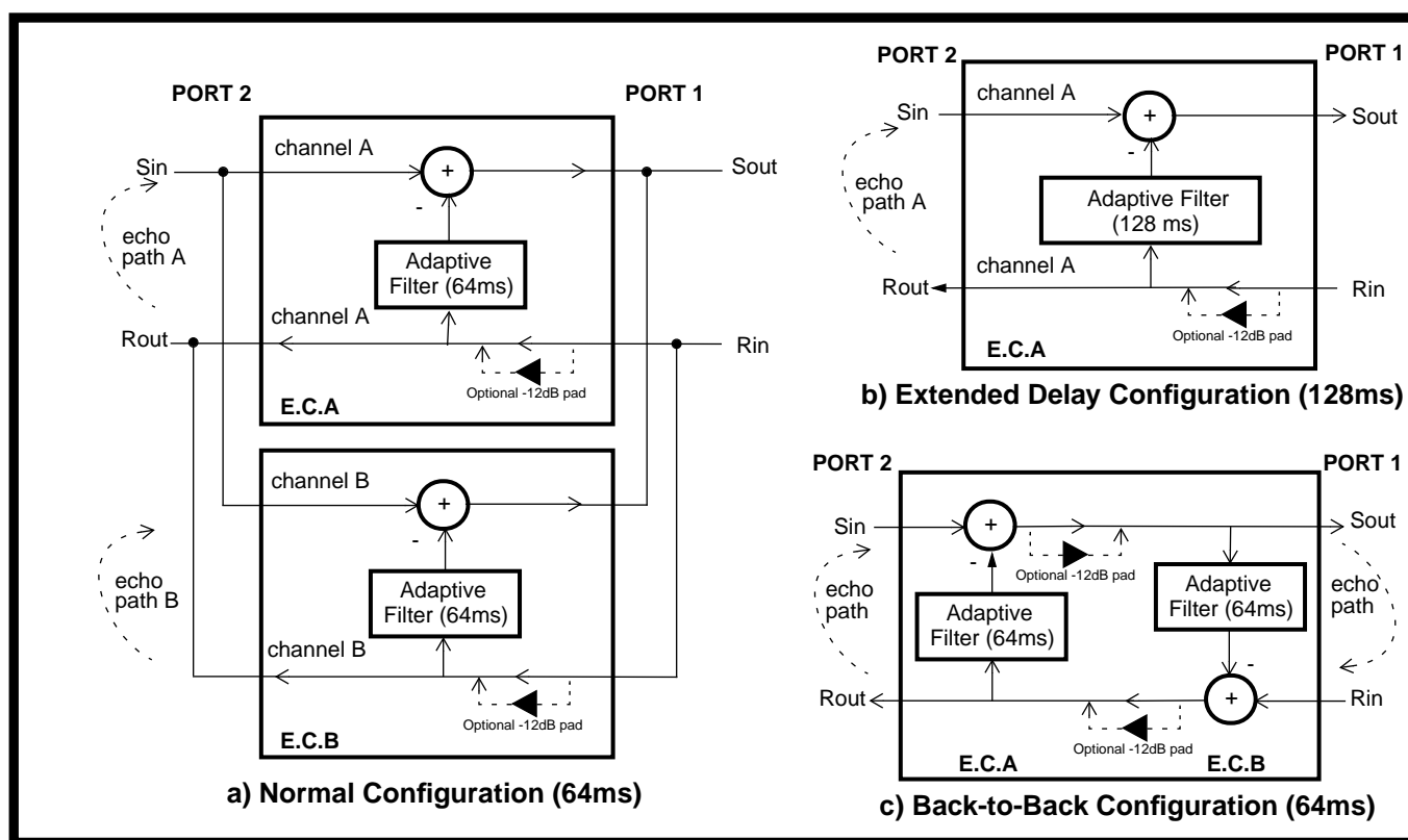
Figure 3 - Device Configuration
