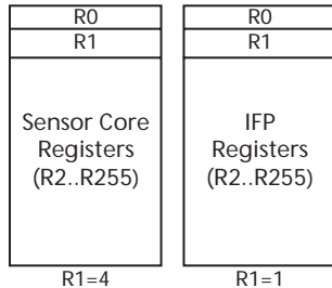
Figure 2: Internal Register Grouping
