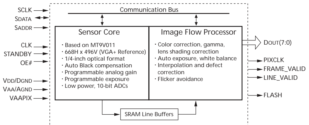
Figure 1: Chip Block Diagram
