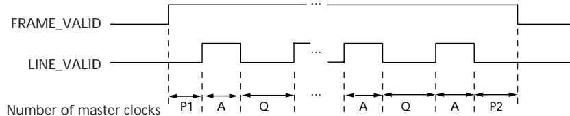
Figure 15: Row Timing and FRAME_VALID/LINE_VALID Signals
