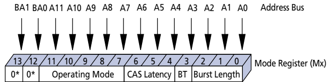
Figure 4: Mode Register Definition Diagram
