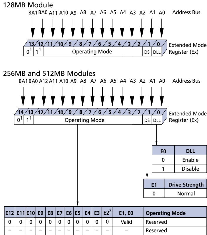
Figure 6: Extended Mode Register Definition Diagram
