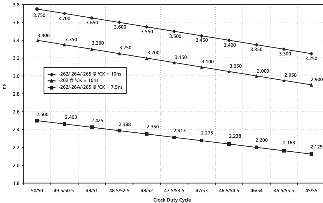
Figure 7: Derating Data Valid Window ( t_{QH} - t_{DQSQ} )
