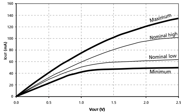
Figure 9: Pull-Up Characteristics
