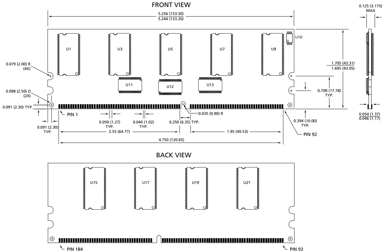
Figure 16: 184-Pin DIMM Dimensions (Low-Profile)
