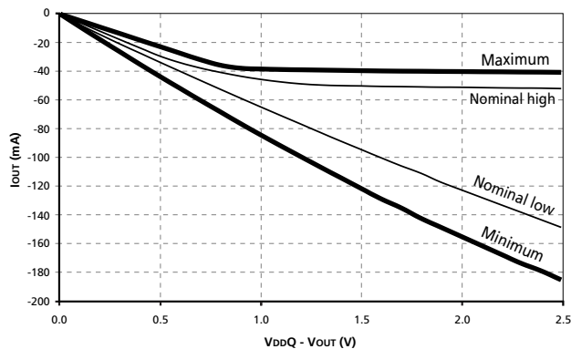
Figure 9: Pull-Up Characteristics
