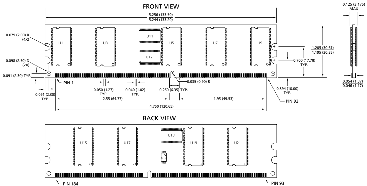
Figure 16: 184-Pin DIMM Dimensions (Low-Profile)
