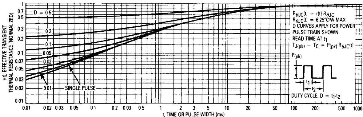
Figure 10. Thermal Response
