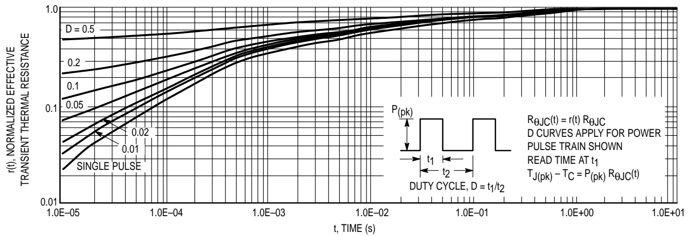
Figure 13. Thermal Response
