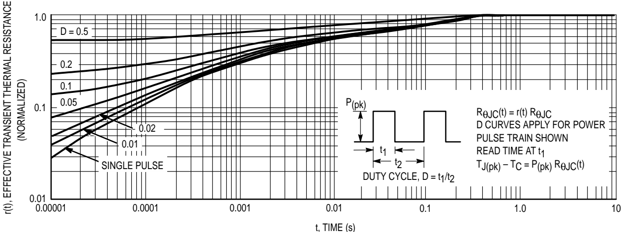
Figure 14. Thermal Response
