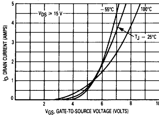
Figure 4. Transfer Characteristics
