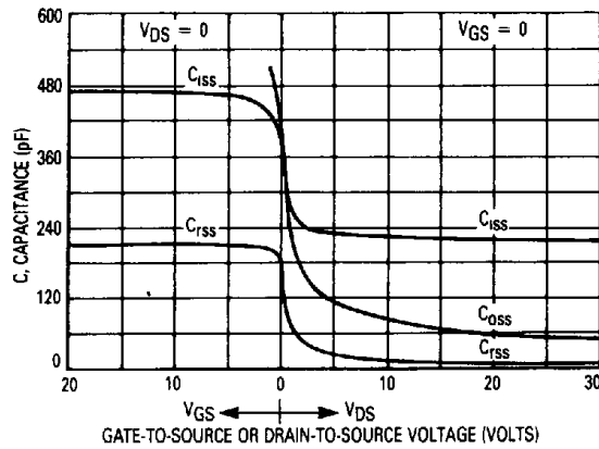
Figure 11. Capacitance Variation
