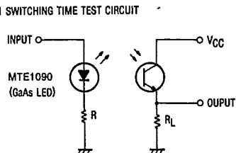
Fig. 1 SWITCHING TIME TEST CIRCUIT
