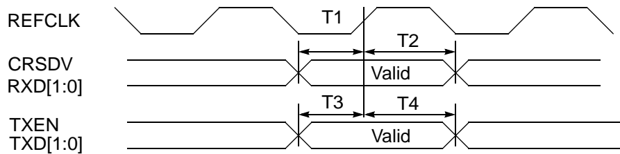
FIGURE 1. RMIi timing
