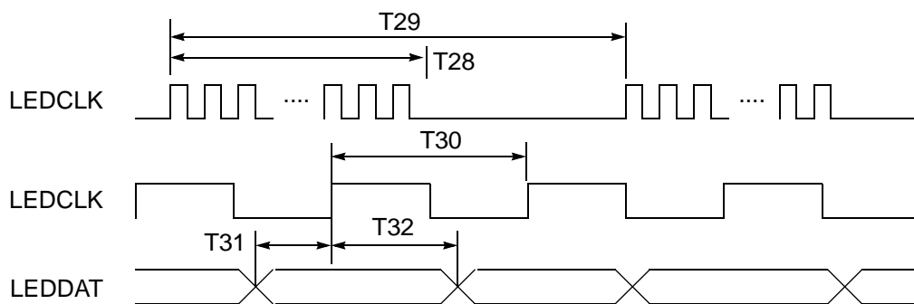
FIGURE 7. LED output timing
