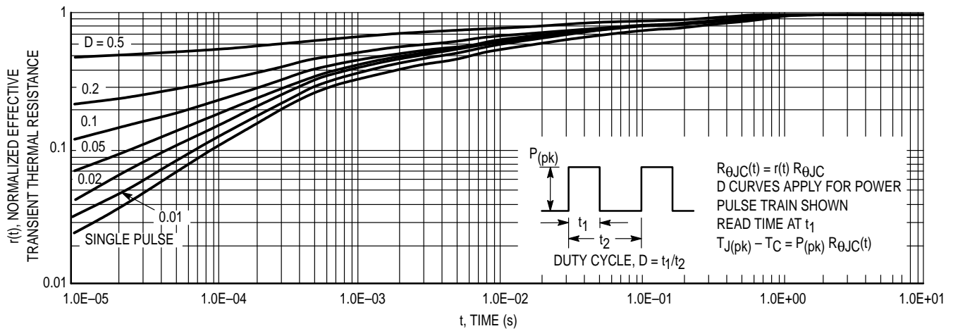
Figure 13. Thermal Response
