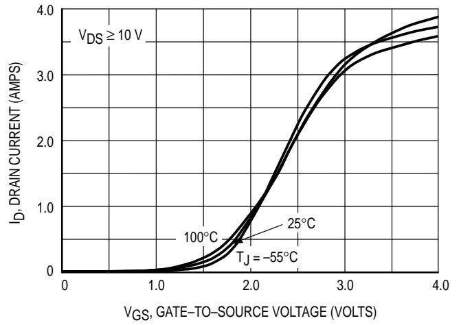
Figure 4. Transfer Characteristics
