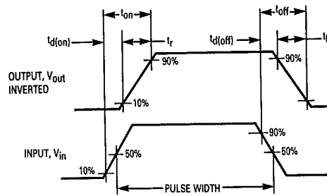
Figure 14. Switching Waveforms
