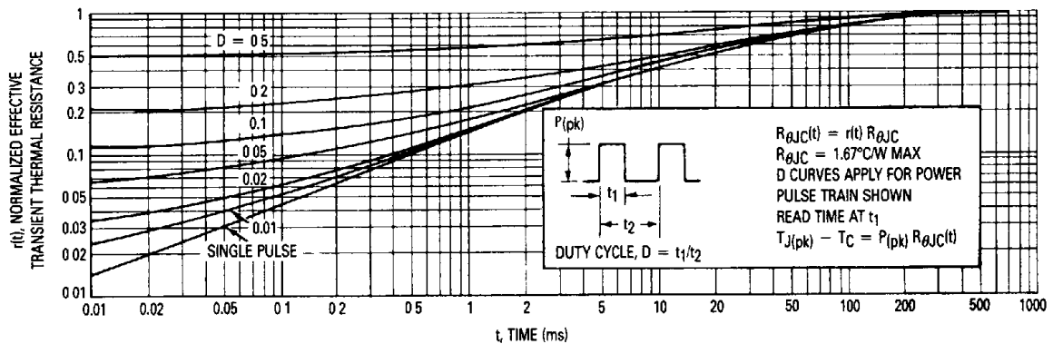
Figure 9. Thermal Response
