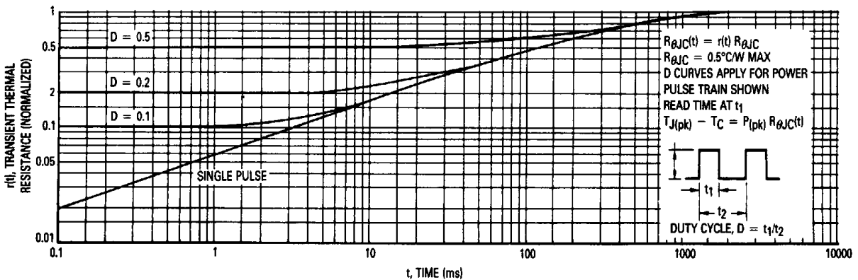
Figure 10. Thermal Response
