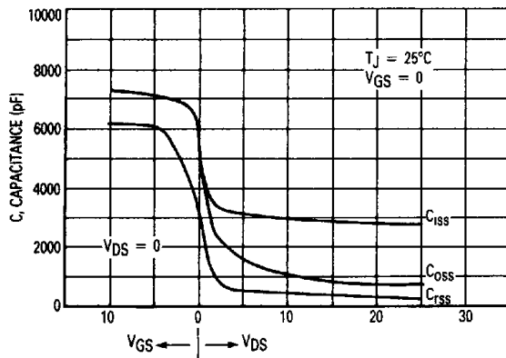
Figure 11. Capacitance Variation
