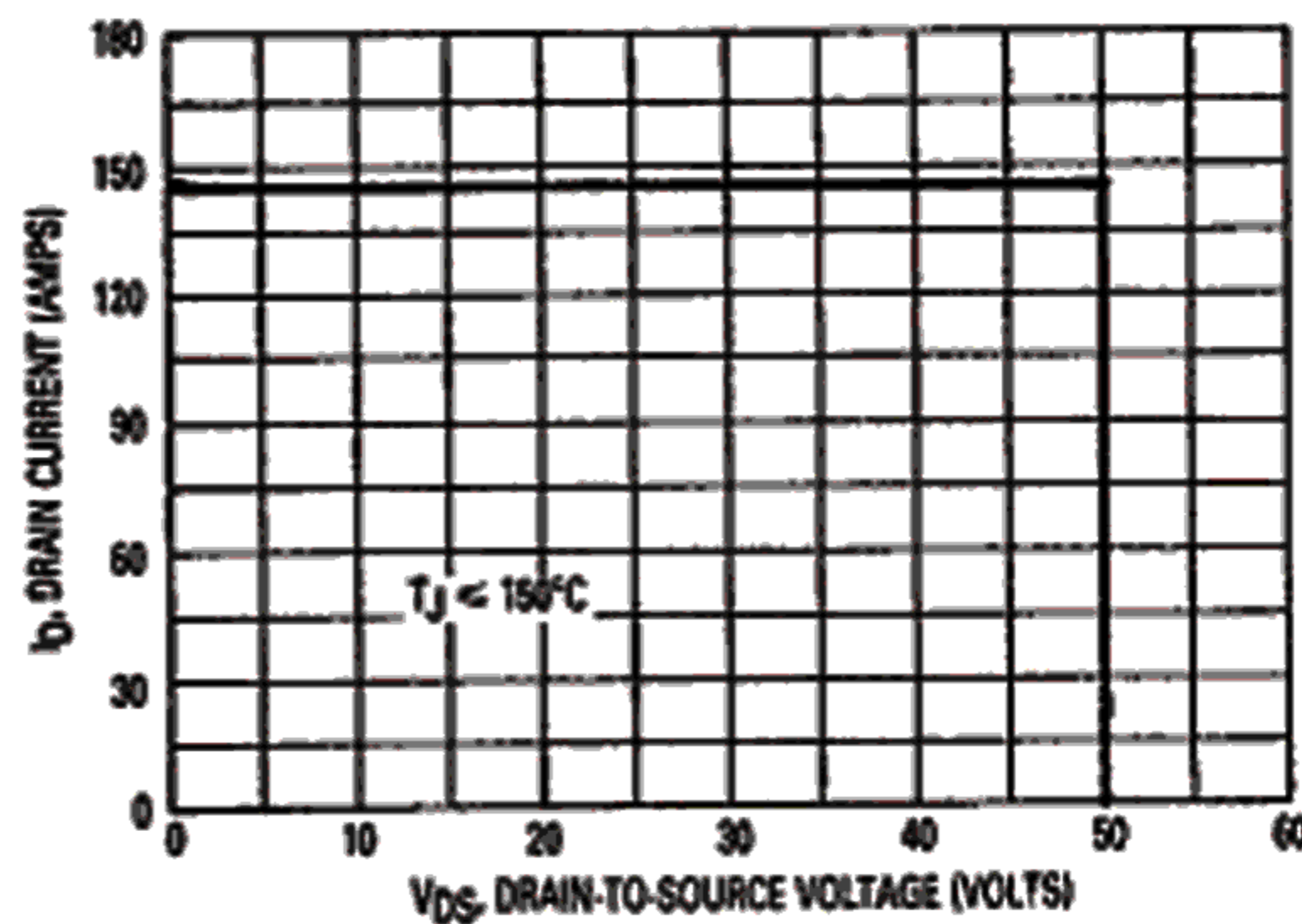
Figure 8. Maximum Rated Switching Safe Operating Area
