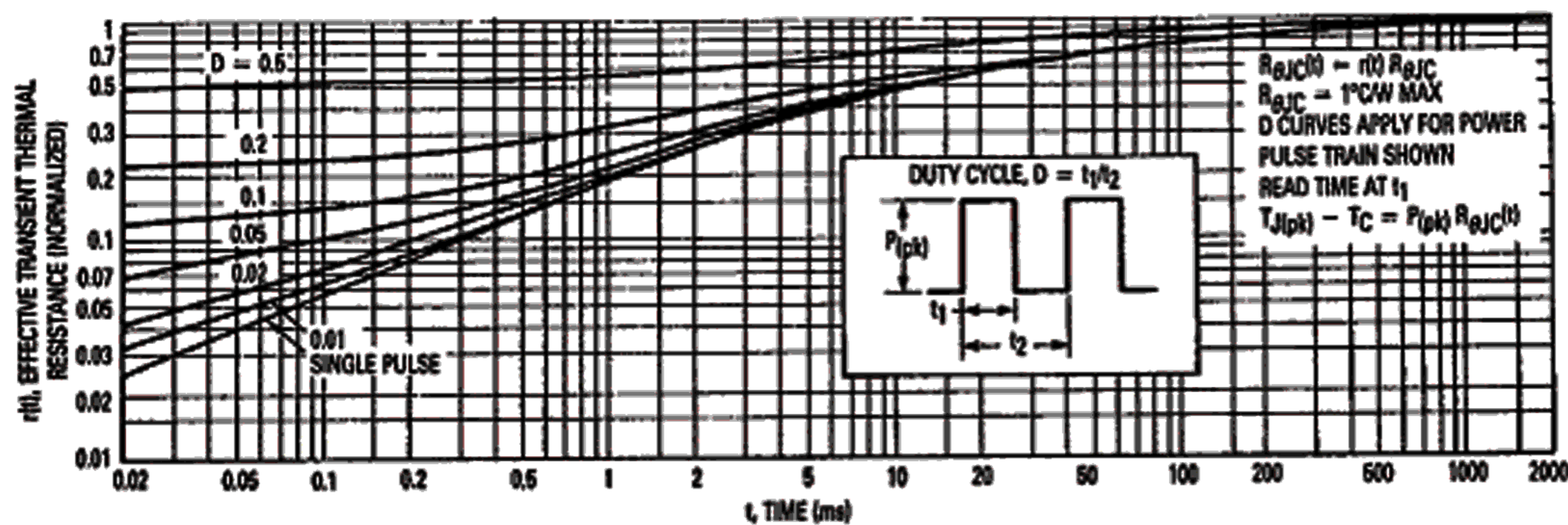
Figure 10. Thermal Response
