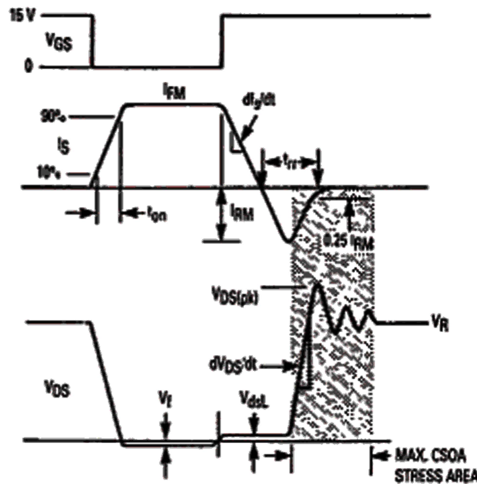
Figure 11. Commutating Waveforms
