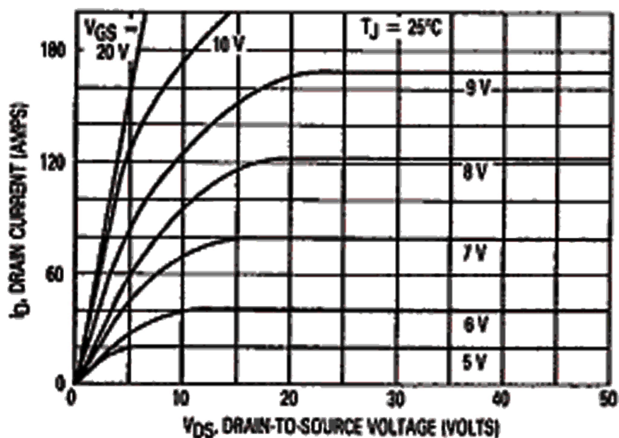
Figure 1. On-Region Characteristics
