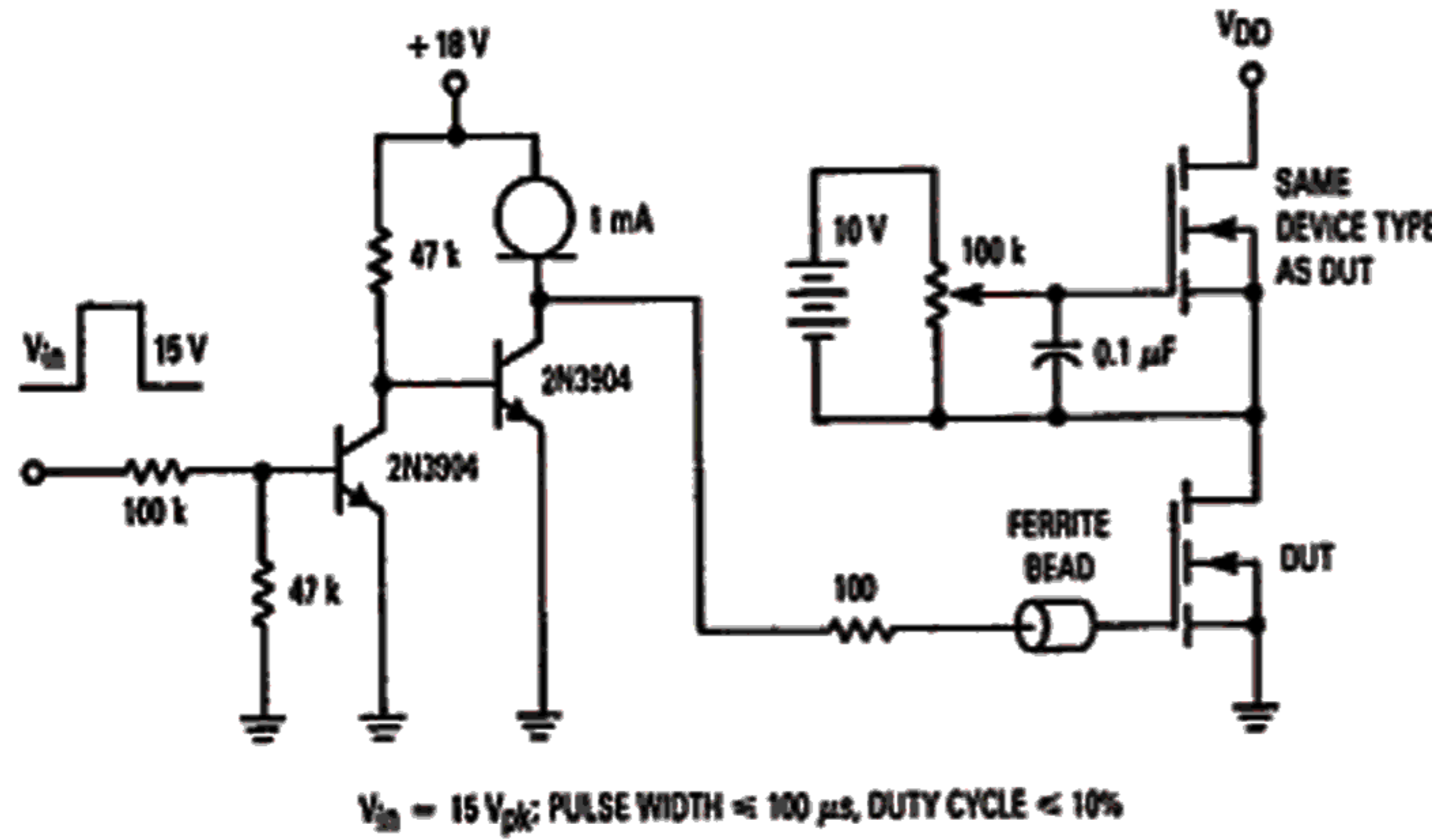
Figure 18. Gate Charge Test Circuit
