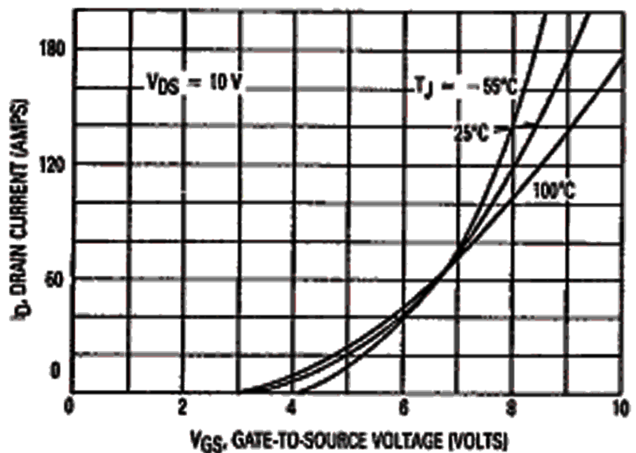
Figure 3. Transfer Characteristics
