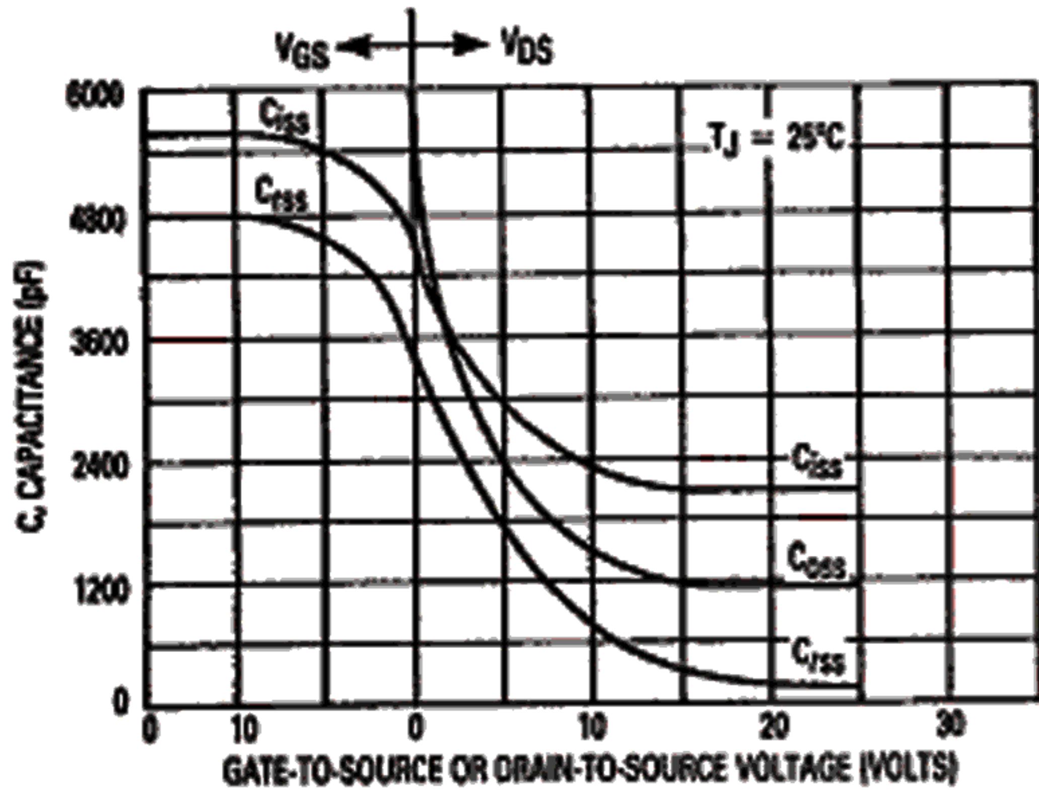
Figure 16. Capacitance Variation
