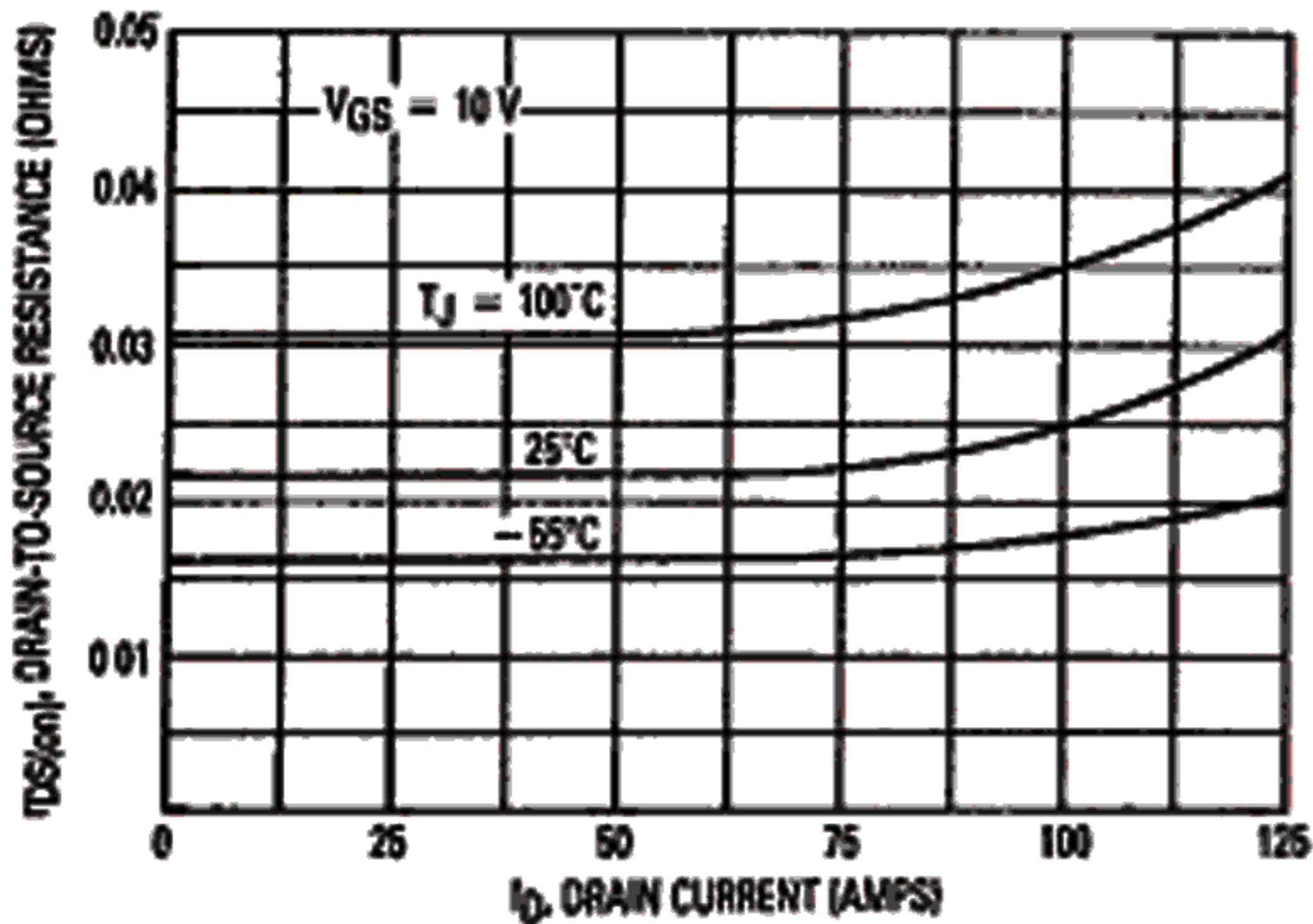
Figure 5. On-Resistance versus Drain Current
