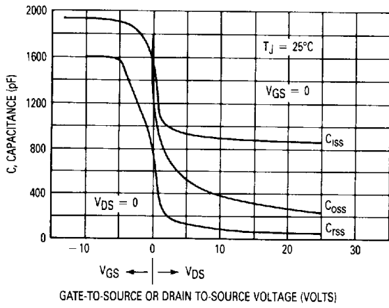
Figure 11. Capacitance Variation
