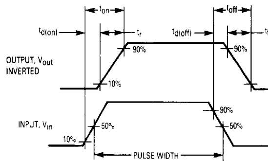
Figure 14. Switching Waveforms
