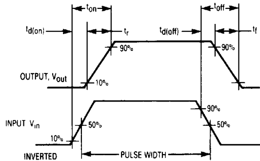
Figure 15. Switching Waveforms
