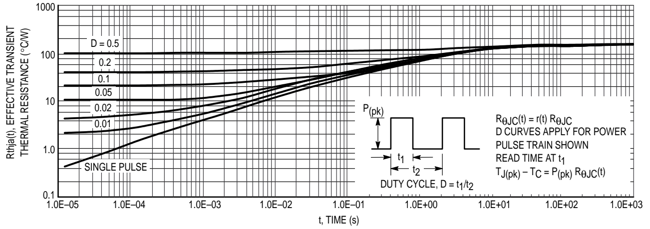
Figure 15. Thermal Response
