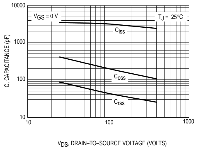
Figure 7b. High Voltage Capacitance Variation
