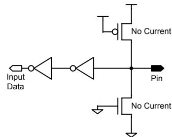
CMOS Pin (Input Mode) Pxxoe=0
