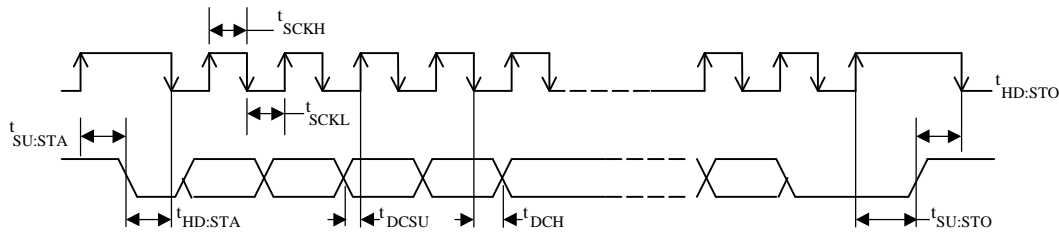
Data interface timing (PC)
