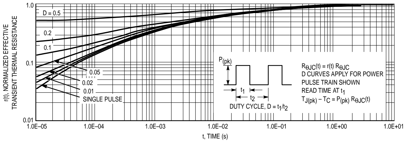
Figure 14. Thermal Response
