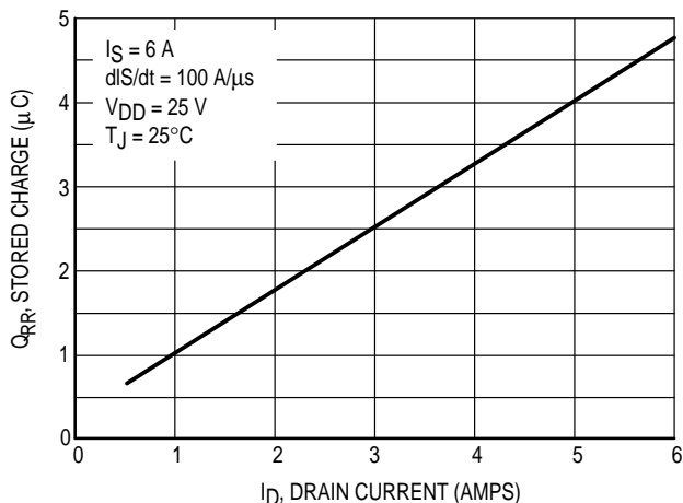
Figure 10. Stored Charge
