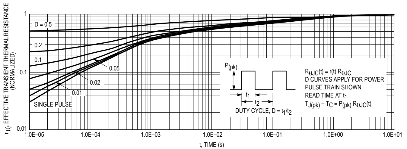
Figure 13. Thermal Response
