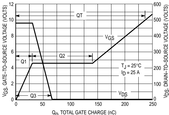
Figure 8. Gate Charge versus Gate-to-Source Voltage
