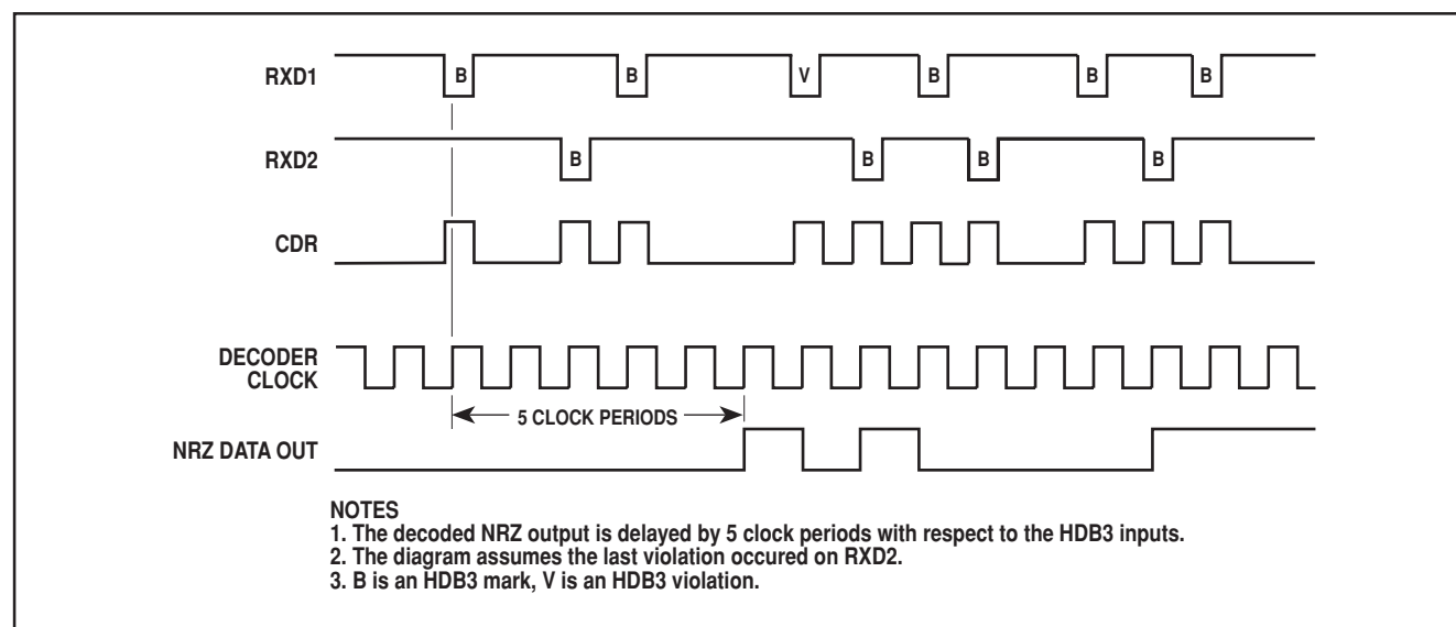
Figure 4 - Decoder waveforms
