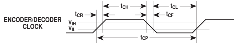
Figure 8 - Clock timing parameters
