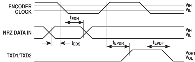
Figure 9 - Encoder timing parameters
