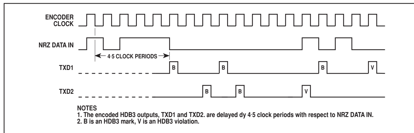
Figure 3 - Encoder waveforms
