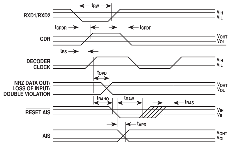
Figure 10 - Decoder timing parameters
