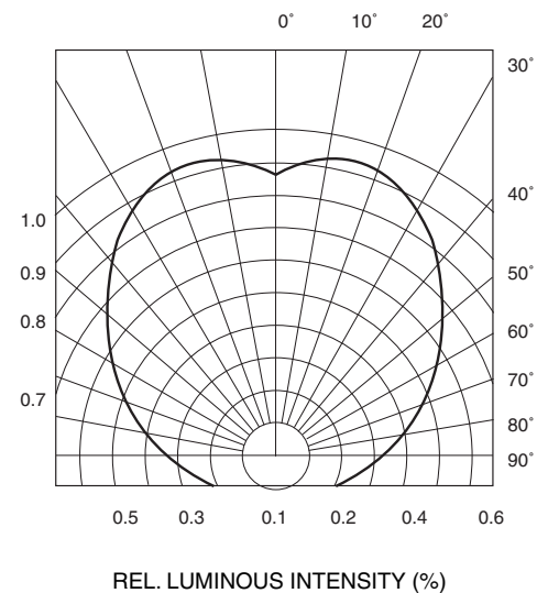
Fig. 4 Radiation Diagram
