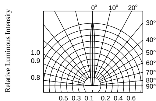
FIG.6 RADIATION DIAGRAM
