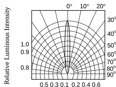
FIG.5 RADIATION DIAGRAM
