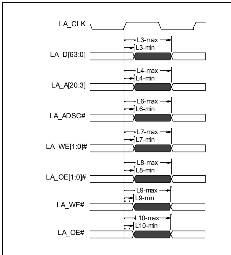
Figure 20 - Local Memory Interface - Output Valid Delay Timing
