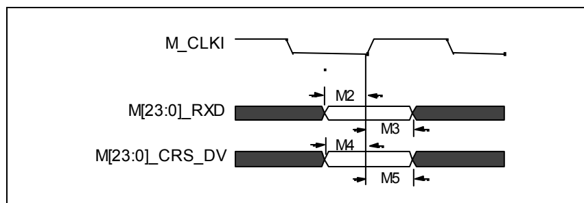
Figure 24 - AC Characteristics – Reduced Media Independent Interface
