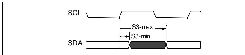
Figure 39 - I 2 C Output Delay Timing
