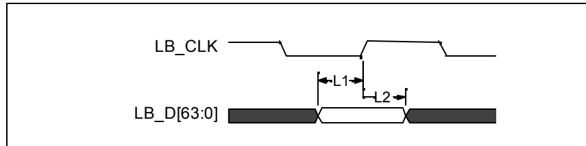
Figure 21 - Local Memory Interface – Input Setup and Hold Timing
