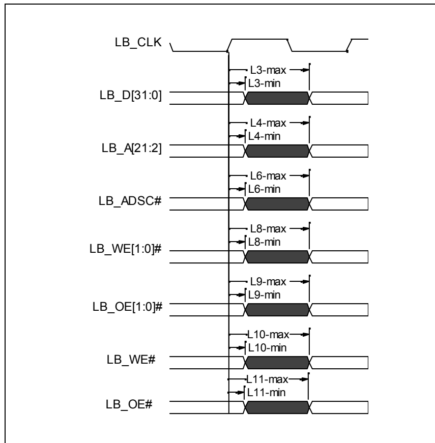
Figure 22 - Local Memory Interface - Output Valid Delay Timing
