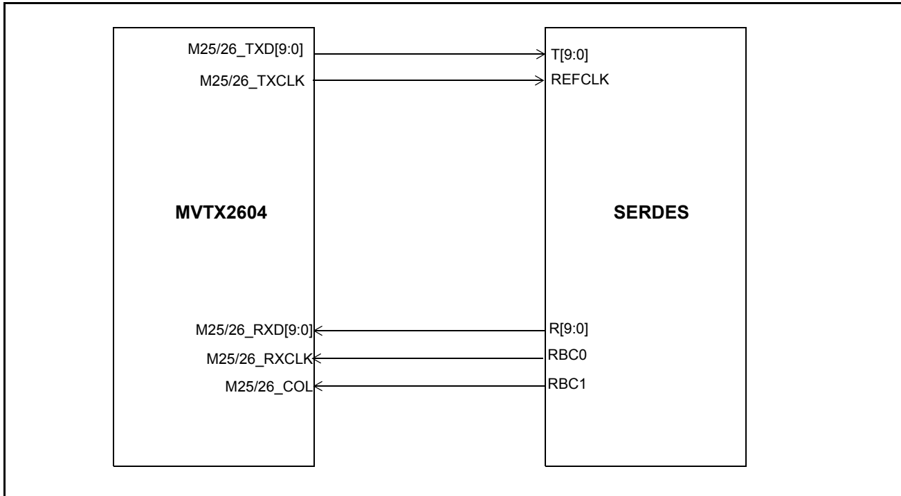
Figure 12 - TBI Connection
