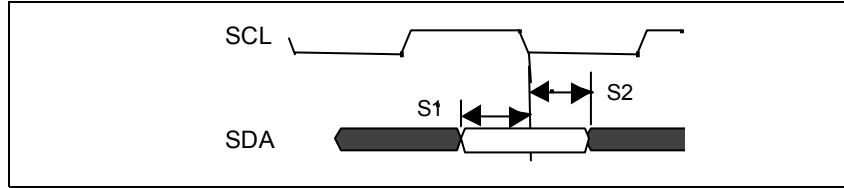
Figure 38 - I 2 C Input Setup Timing
