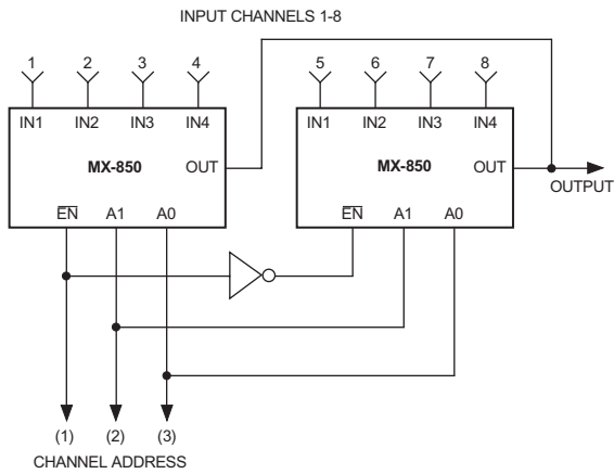
Figure 6. Cascading Multiple MX-850's
