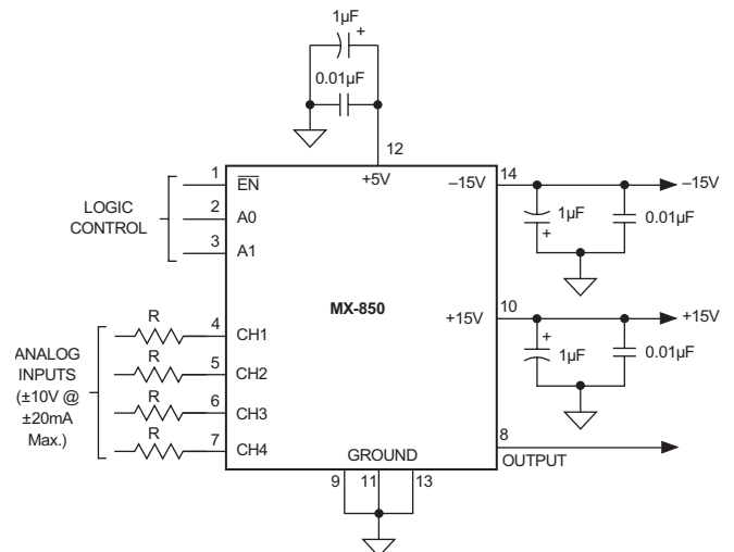
Figure 5. Typical Connections
