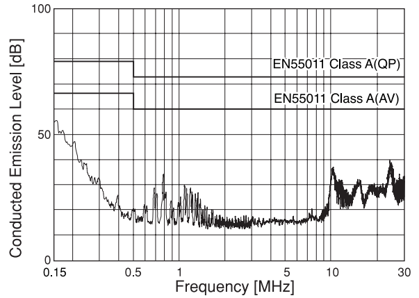
● Machine with Servo Driver + MX13050
