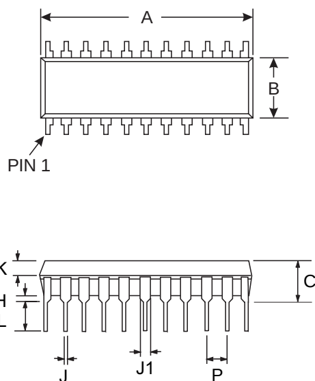
Figure 14: 22-pin PDIP Mechanical Outline: Order as part no. MX469P
