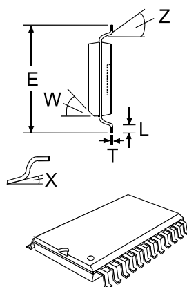
Figure 13: 24-pin SOIC Mechanical Outline: Order as part no. MX469DW
