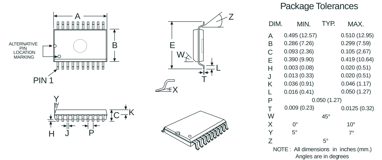
Figure 15: 20-pin SOIC Mechanical Outline: Order as part no. MX469D3
