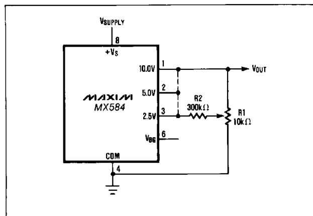
Figure 3. Fine Adjustment of Output Voltage ( \pm 200mV )
