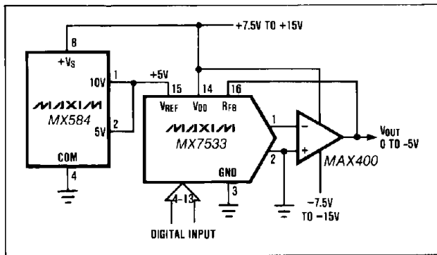
Figure 10. Low Power 10 Bit CMOS DAC Connection
