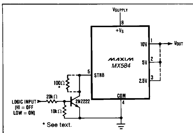
Figure 5. Use of Strobe Terminal
