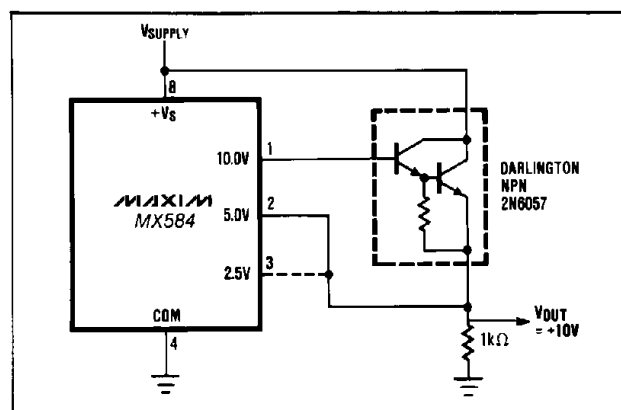
Figure 7. NPN Output Current Booster
