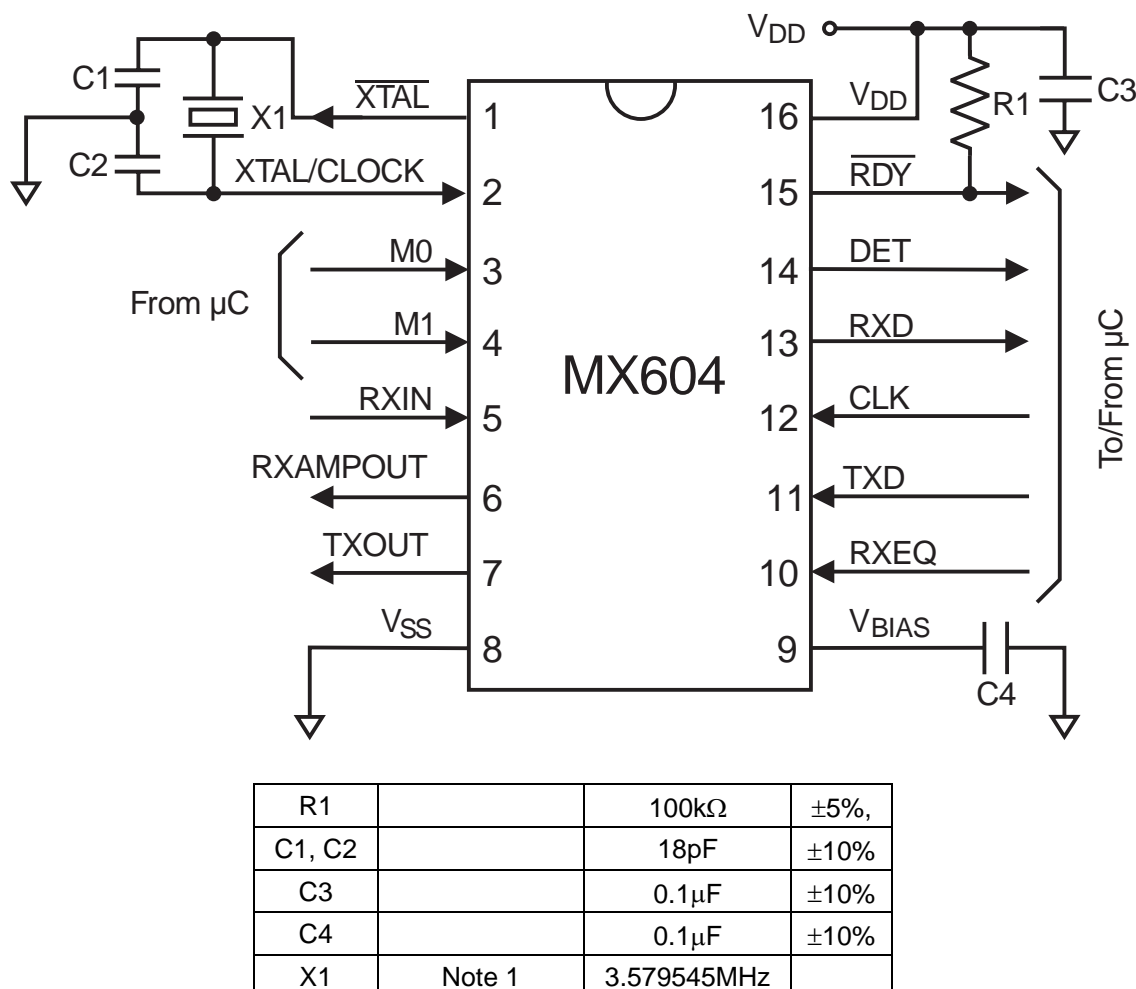
Figure 2: Recommended External Components for Typical Application
