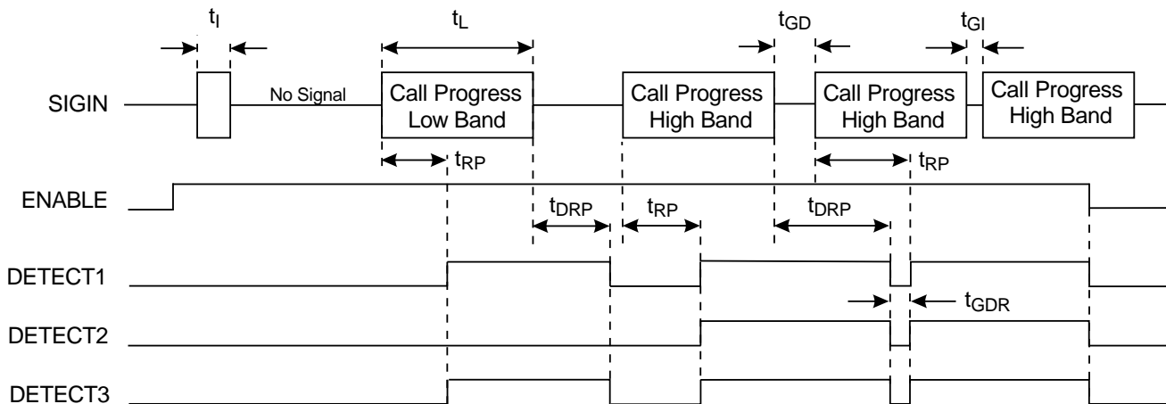
Figure 3: Timing Diagram: Call Progress Tone(s)
