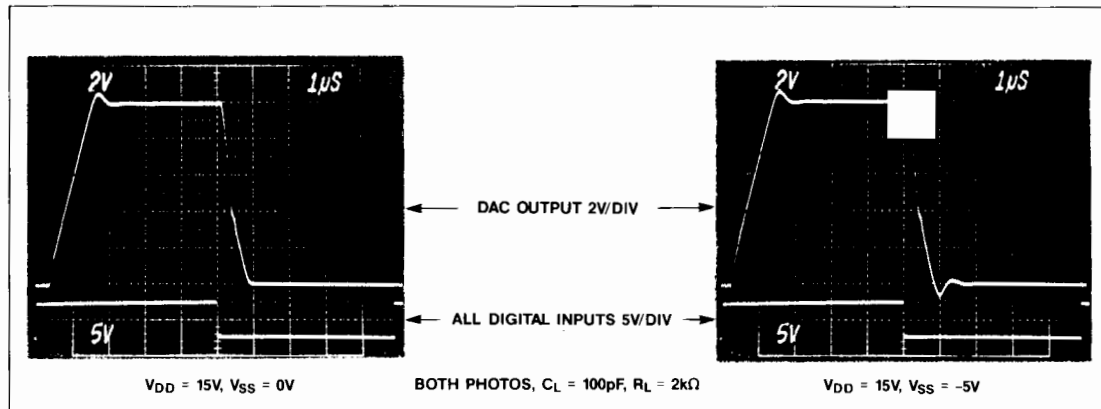
Figure 3. Dynamic Response
