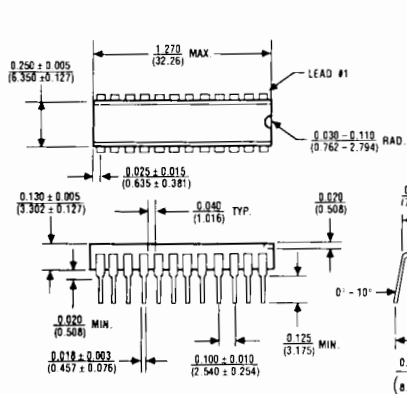
24 Lead Plastic Narrow DIP (NG)
