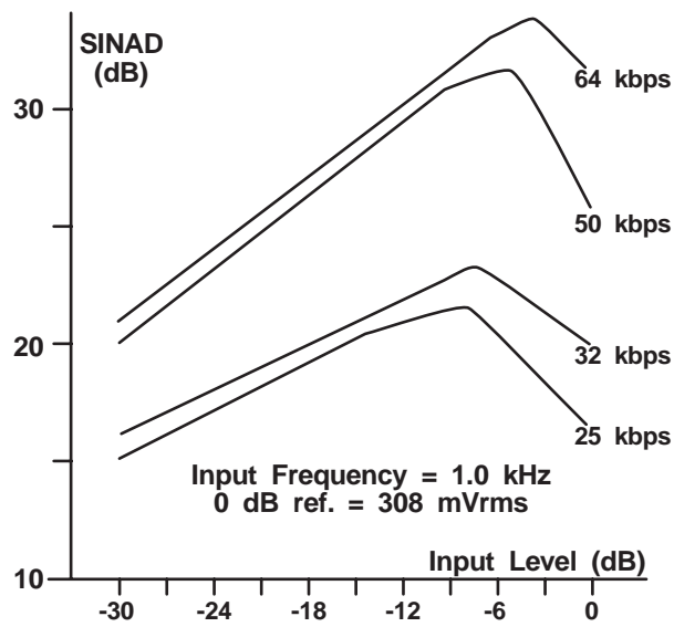
Figure 6: SINAD vs. Input Level at Different Sample Rates
