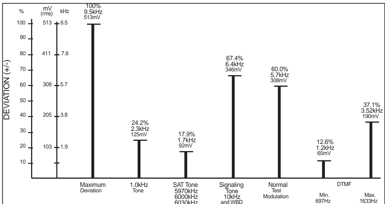
Figure 4 - Signal Deviation Levels and corresponding TX Mod Outputs with the Mod Level set to 0dB
