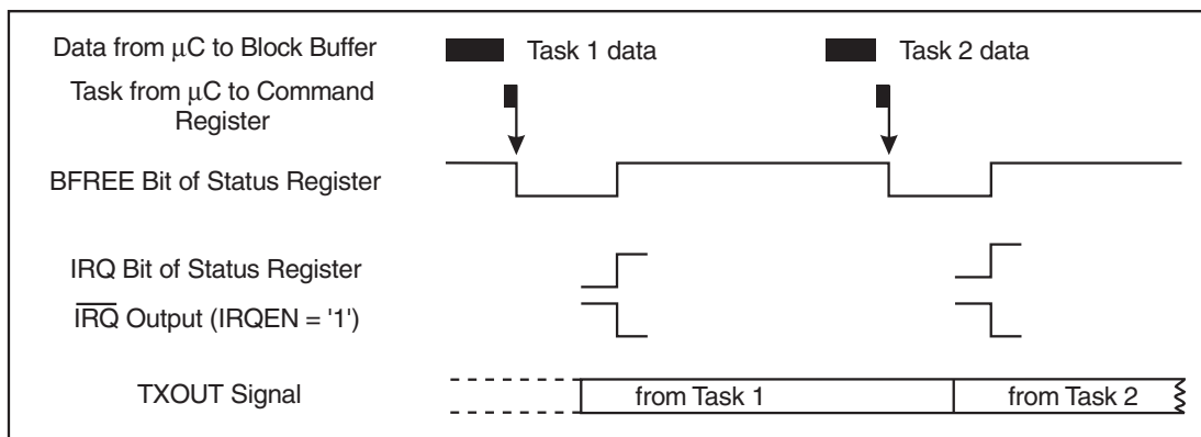
Figure 9: Transmit Task Overlapping
