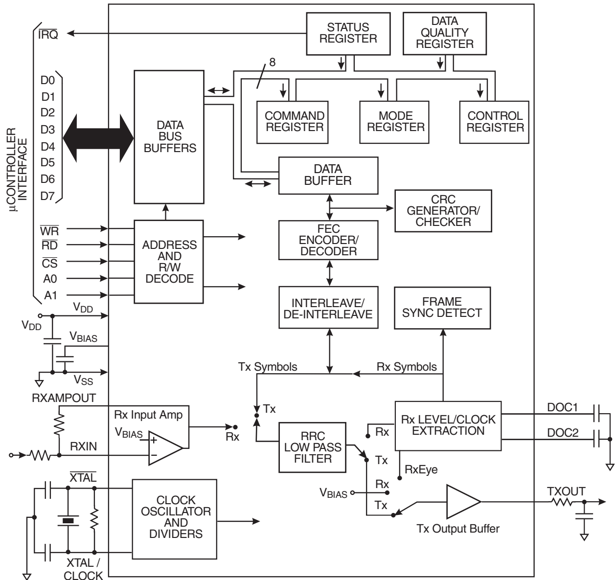
Figure 1: Block Diagram
