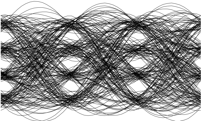
Figure 18: Tx Signal Eye TXIMP = 1
