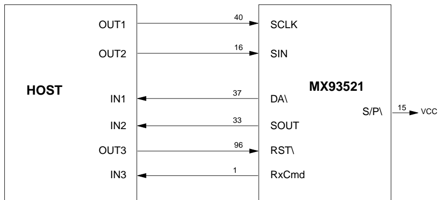
SERIAL MODE
