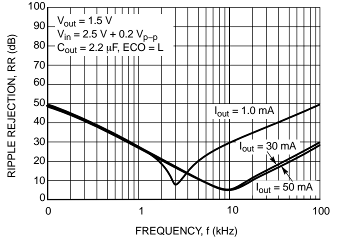
Figure 28. Ripple Rejection vs. Frequency
