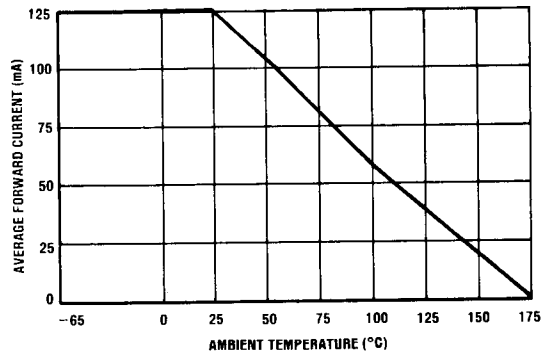
FIGURE 3 HVE/HVE 40-100/1N5181-84
