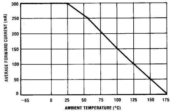
FIGURE 2 HVE/HVE 10-30/1N3643-47
