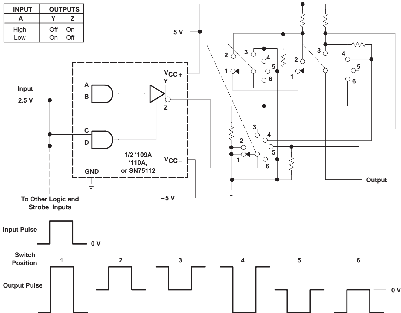
Figure 5. Pulse-Control Circuit
