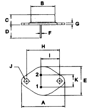
TO-66
