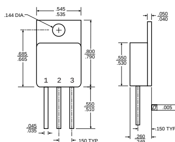
TO-254AA
