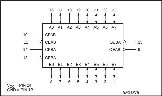
LOGIC SYMBOL – 74F2952
