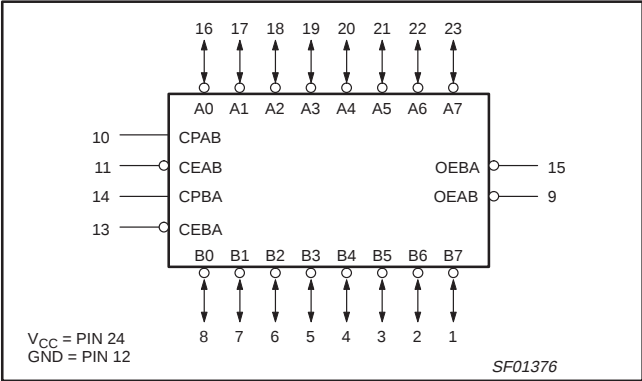
LOGIC SYMBOL – 74F2953
